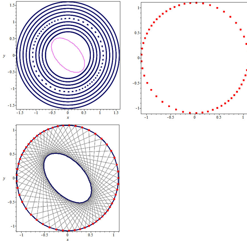
Fig. 3 (a) 5000 iterates of F with the grid of initial conditions \mathcal{S} . (b) 19950 iterates with initial condition (1.1000045, 0) . (c) The Poncelet's construction of the 57-periodic orbit.
