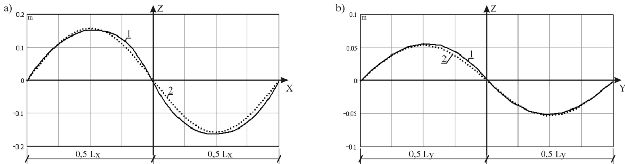
Figure 5. Displacements of the surface under an inverse-symmetric load: a – the section by the plane (XOZ), b – the section by the plane (YOZ); 1 – curves, obtained with the help of the special computer program EASY, 2 – curves, calculated with the formula (11)
