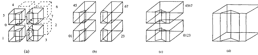
Figure 3. The reduction of a set of Face nodes to an Edge. The merging process starts grouping these descendants by pairs (n_0, n_1), (n_2, n_3), (n_4, n_5) and (n_6, n_7) . At this first step the Plane Position test hasn't to be applied, the resultant configuration can be obtained from the MT table directly (see Table 2, where (N, F) \rightarrow F ). The resultant configurations \{F, F, F, F\} are grouped again and evaluated. In this case, the Plane Position test has to be applied to select if the pair (F, F) generates a Face, an Edge or a Band n . As planes intersected into the node, the generated codifications are Edges. Finally, (n_{0123}, n_{4567}) is evaluated. In this case, the (E, E) configurations generate an Edge.
