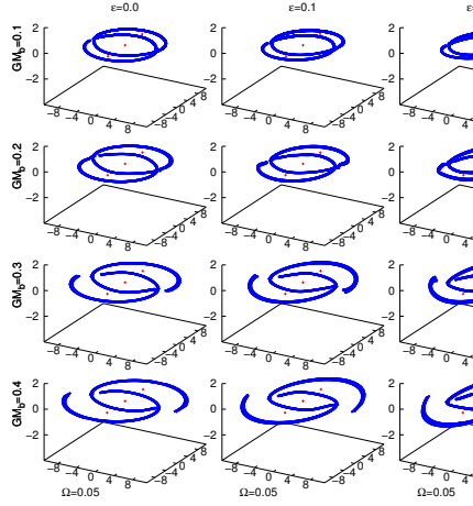
Figure 14: As in Fig. 12 in a 3D view.
