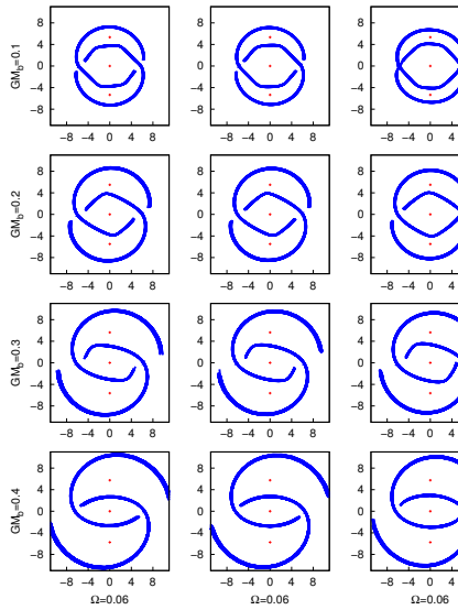
Figure 13: As in Fig. 12 for \Omega = 0.06 .
