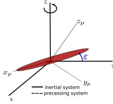
Figure 3: Reference systems. The major axis of the bar is aligned with the precessing x axis and the precessing z axis describes a cone about the inertial Z axis. Here (x_p, y_p, z_p) denotes the precessing reference frame and (X, Y, Z) the inertial one.
