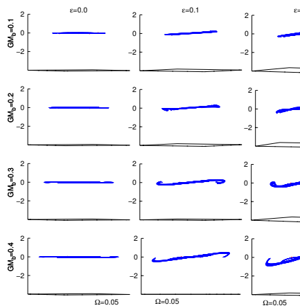
Figure 16: As in Fig. 12 but in the side-on view.
