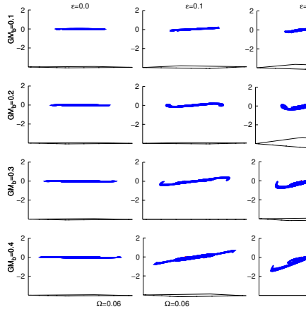
Figure 17: As in Fig. 13 but in the side-on view.
