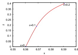
Figure 6: Variation of the xz coordinates of L_1 as \varepsilon varies within the range \varepsilon \in [0, 0.2] for the precessing model with GM_b = 0.1 . The marked dots show the L_1 coordinates for three specific values of \varepsilon : \varepsilon = 0 (bottom part of the plot) \varepsilon = 0.1 (middle) and \varepsilon = 0.2 (top).
