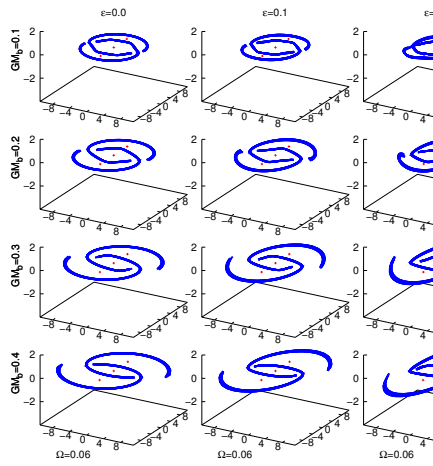
Figure 15: As in Fig. 13 in a 3D view.
