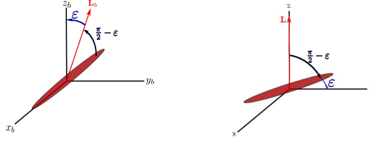
Figure 2: Reference systems. Top: Bar in the body reference frame, where the angular momentum \mathbf{L}_b and the y_b z_b plane keep an angle \epsilon . Bottom: Bar in the inertial reference frame, where the angular momentum is aligned with the Z axis and the major axis of the bar keeps an angle \epsilon with the XY plane.
