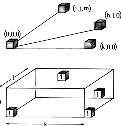
Figure 9. The construction of the three dimensional lattice • La construction du treillis tridimensionnel.
