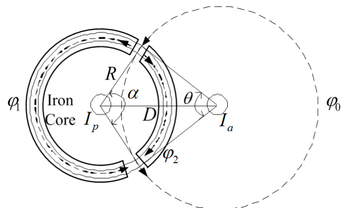
Magnetic circuit model in hypothetical equivalently homogeneous medium
