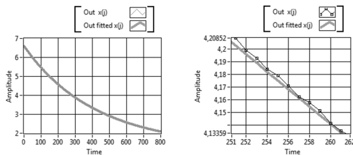
Estimation results based on the ML method for multiexponential signal with and without superimposed noise
