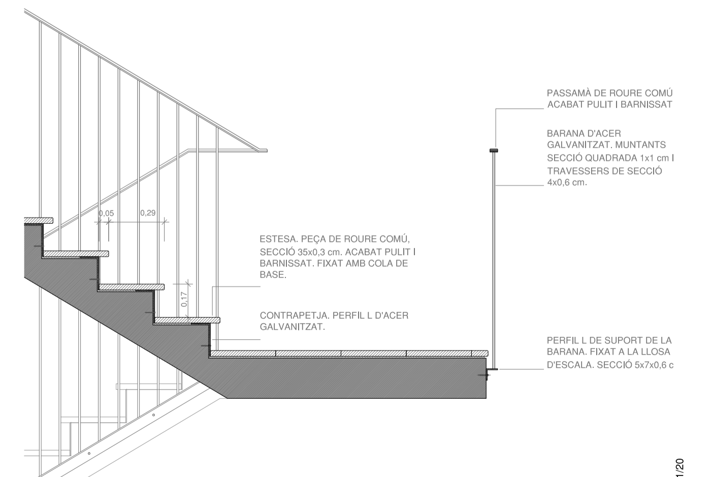
DETALLS_MATERIALS ACABAT 1/20
