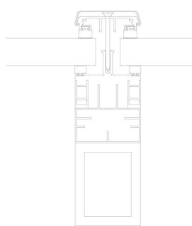
Detalle lucernario
