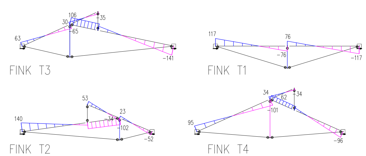
7 - Diagrama de tallants (sense majorar) [kN]
