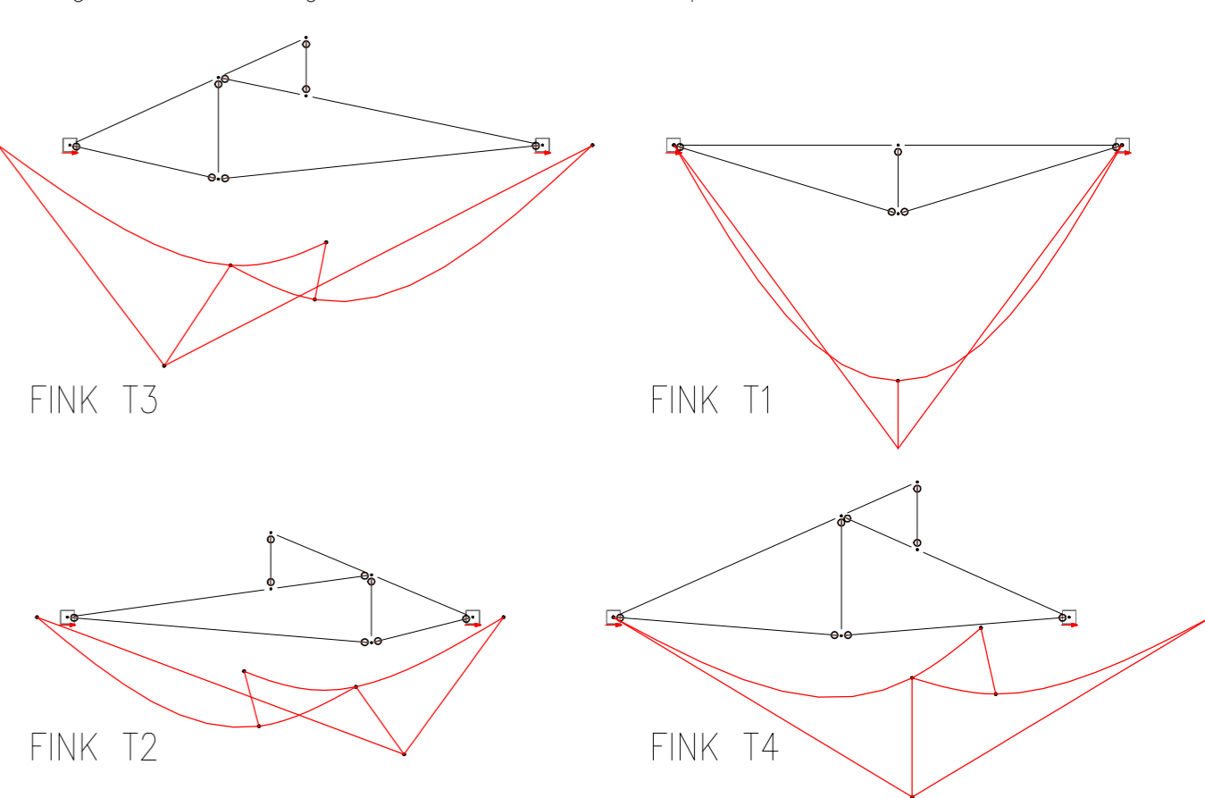
5 - Diagrama d'axils (sense majorar) [kN]
