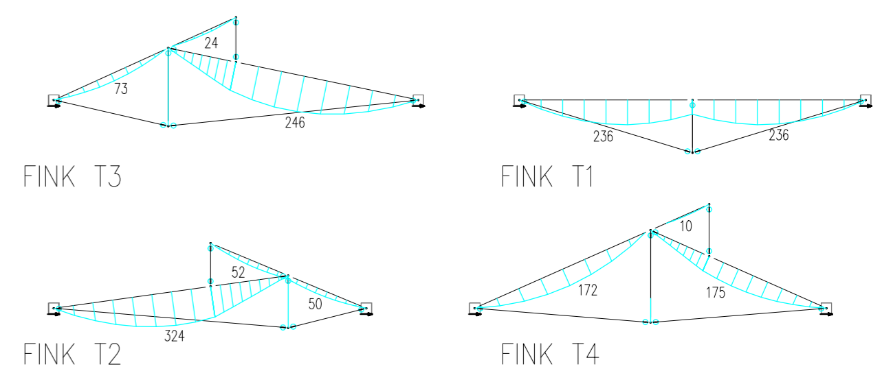
7 - Diagrama de tallants (sense majorar) [kN]
