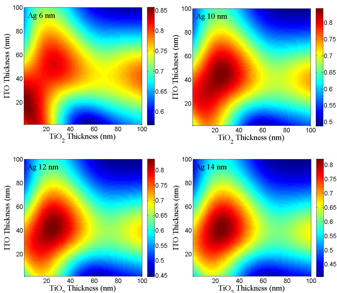
Fig. S1. Simulated mean visible transmittance between 375-700nm for different thicknesses of bottom \text{TiO}_2 and top ITO layer for (a) Ag 6nm, (b) 10nm, (c) 12nm, (d) 14nm
